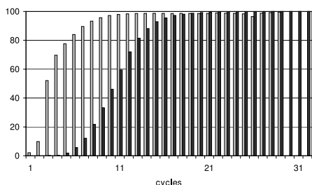
Figure 6: Event dissemination. Light bars show the hit ratio for non-complete disseminations. Dark bars show the percentage of disseminations that were complete (events delivered to all their matching subscribers). 10K nodes; 3 attributes; power law interest distribution.
